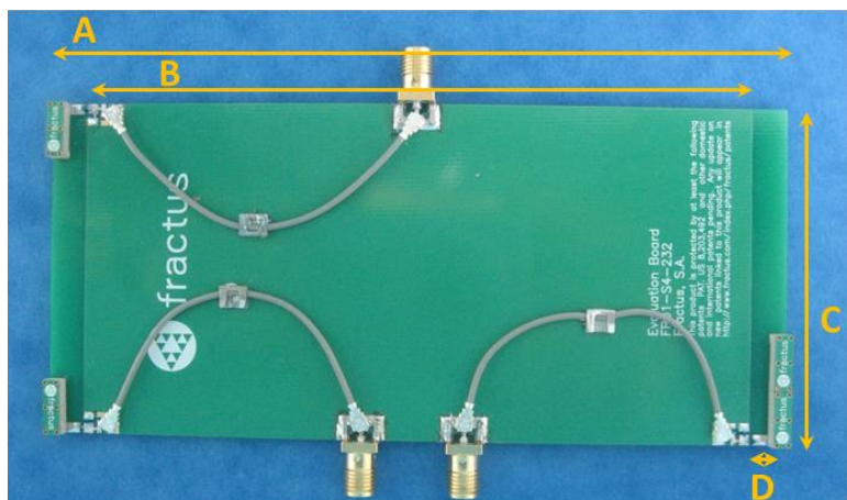
Figure 1 – EB_FR01-S4-232-UFL3R. Evaluation Board providing operation in 3 frequency ranges, 698 MHz to 798 MHz, 824 MHz to 960 MHz, and 1710 MHz to 2690 MHz.
