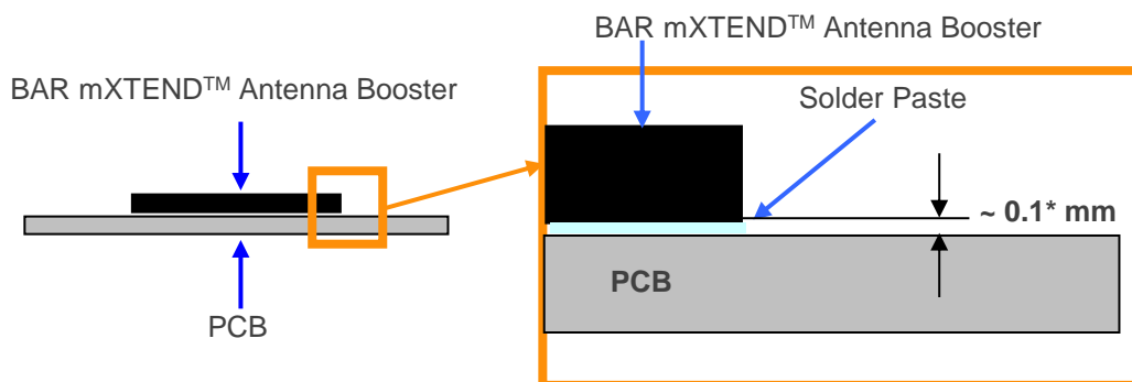
Figure 12 – Soldering Details.
